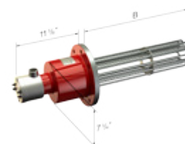
5 inch ANSI flanged heater NEMA 7
