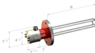
3 inch ANSI flanged heater NEMA 4
