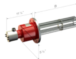
4 inch ANSI flanged heater NEMA 7
