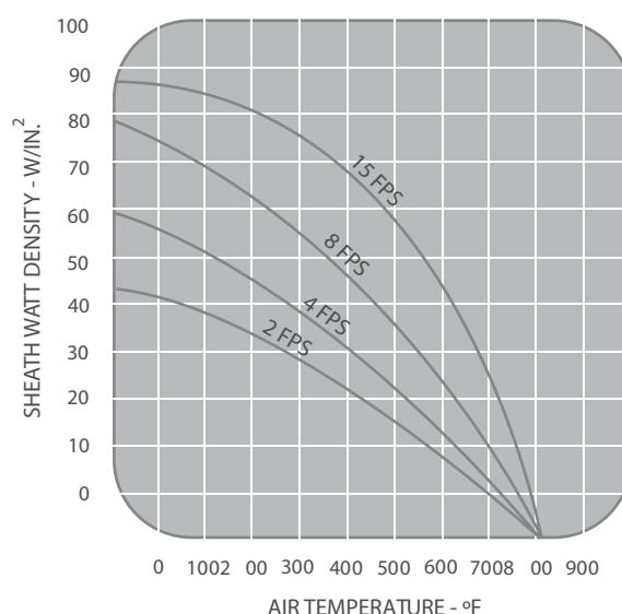
FIG. 1 - Watt Density vs. Air Temperature for 797°F (425°C) Fin Temperature
